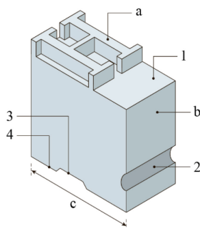
Figure 1. Type structure: a – face, b – body or shank, c – point size; 1 – shoulder, 2 – nick, 3 – groove, 4 – feet Source: Jensen (2006), CC0.
